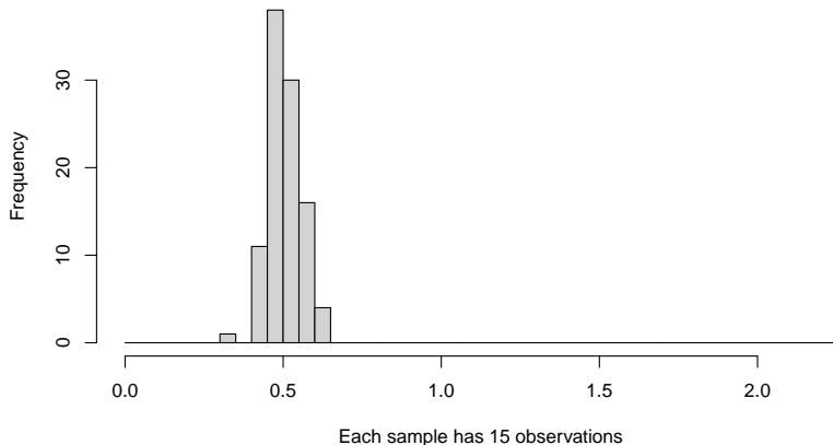
Sampling Distribution, 100 Sample Means
